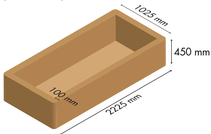
Knee-height raised beds (0.45 m tall)
